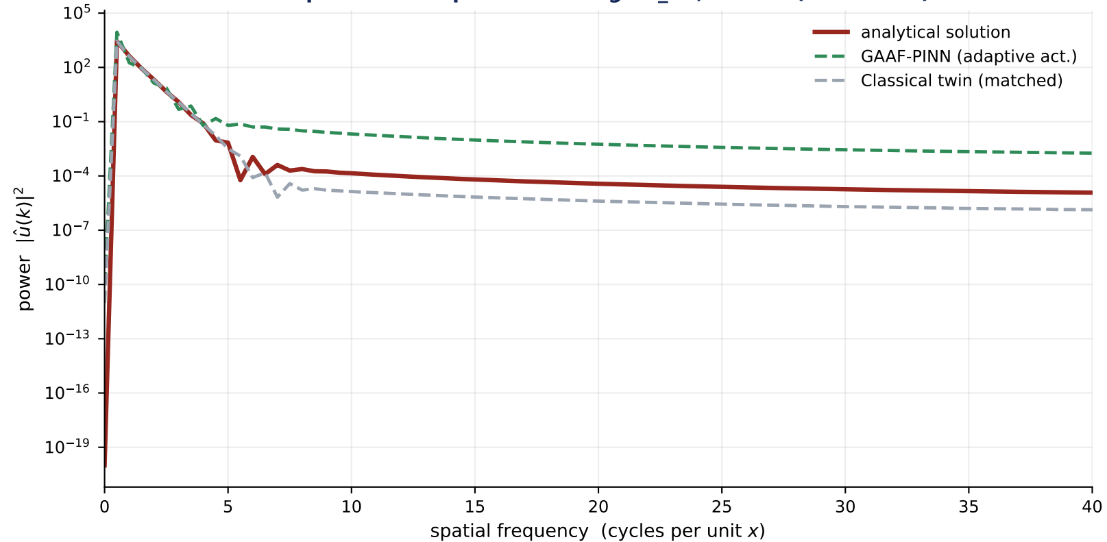
Output Fourier spectrum - burgers_n3, t = 1.00 (seed 1234)
